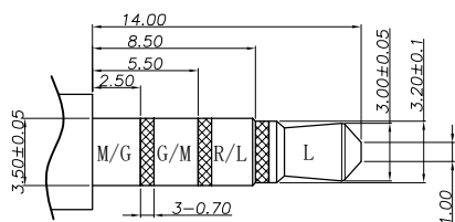
RECOMMENDED PLUG ø3.5 4-POLEPLUG(TOL±0.05)
